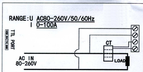
Figure 1 Wiring diagram
